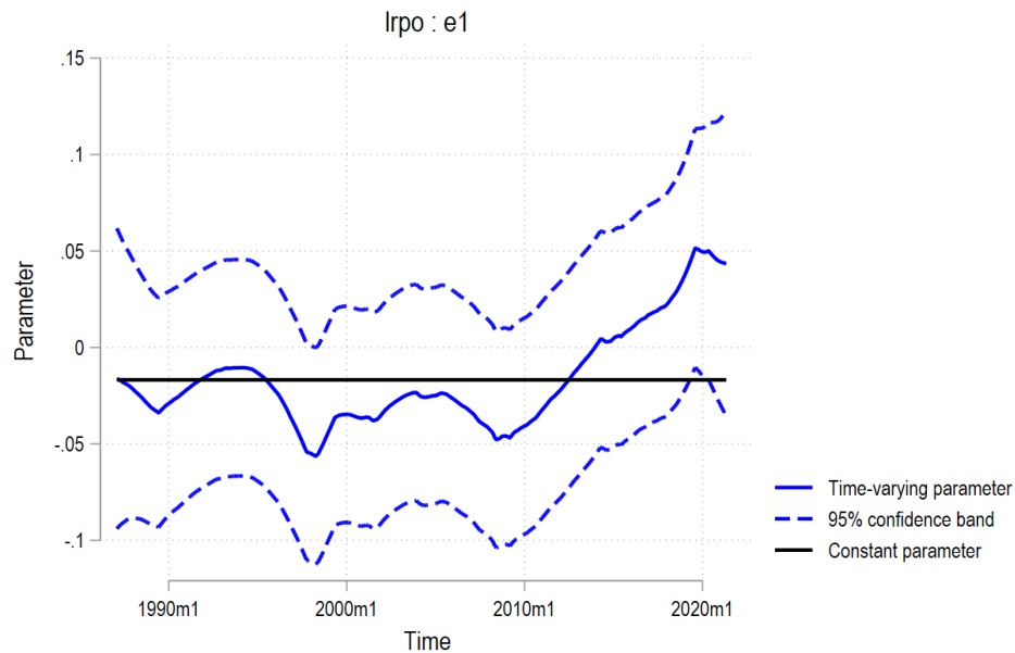
Figure 4. Time-varying parameter plot at horizon T = 8
